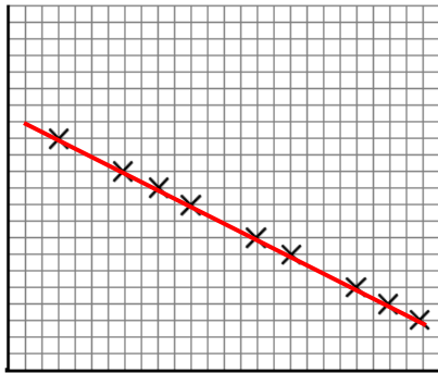
Perfect negative correlation
