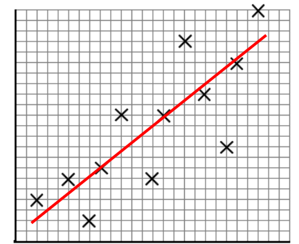
Weak positive correlation
