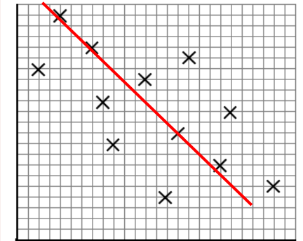
Weak negative correlation
